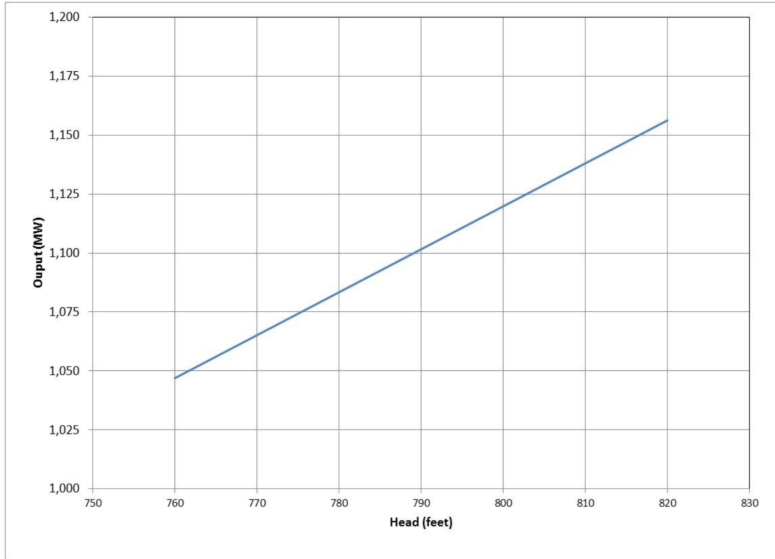
Figure 3.6-3. Northfield Mountain Pumped Storage Development - Plant Capability (MW) versus Head (ft) Curve
