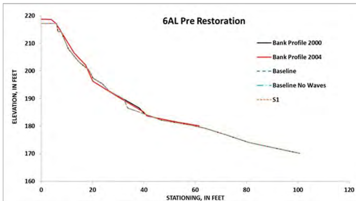
Figure 5.4.3.16-2: Simulated, future unit-erosion for the Baseline Condition (with boat waves on and off) and Scenarios 1 at site 6AL for the period 2000-2004
