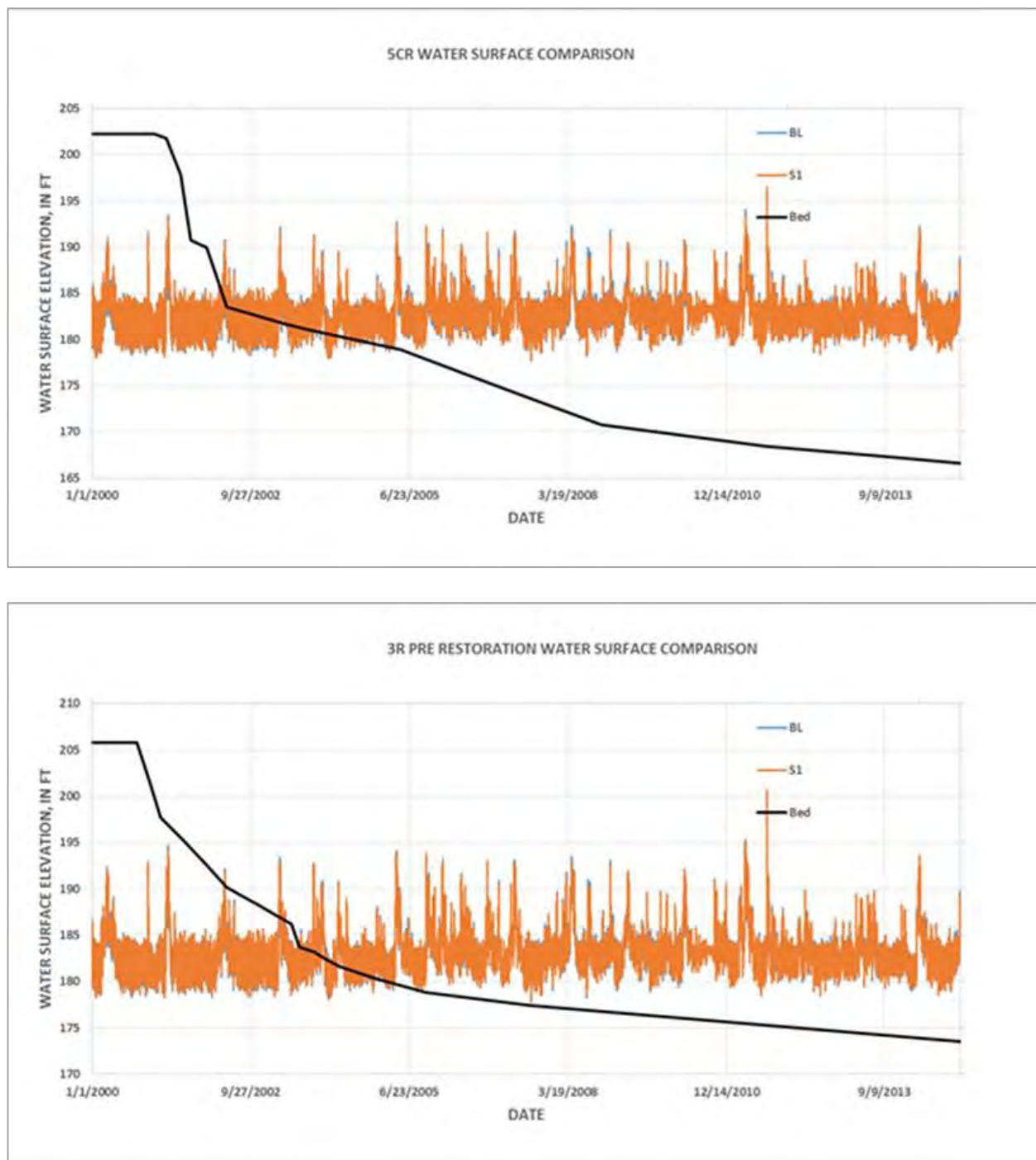
Figure 5.4.1.1-5 Water-surface elevations for representative sites within the Middle Reach (#3; site 5CR) and Upper Reach (#4; site 3R Pre-restoration)
