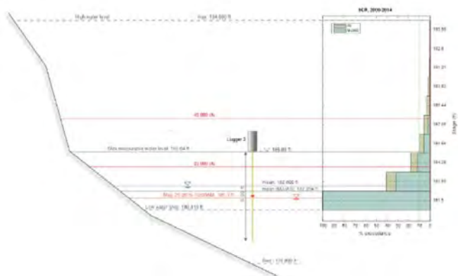
Figure 4.2.8.2-7 WLOG-2 installation elevation
