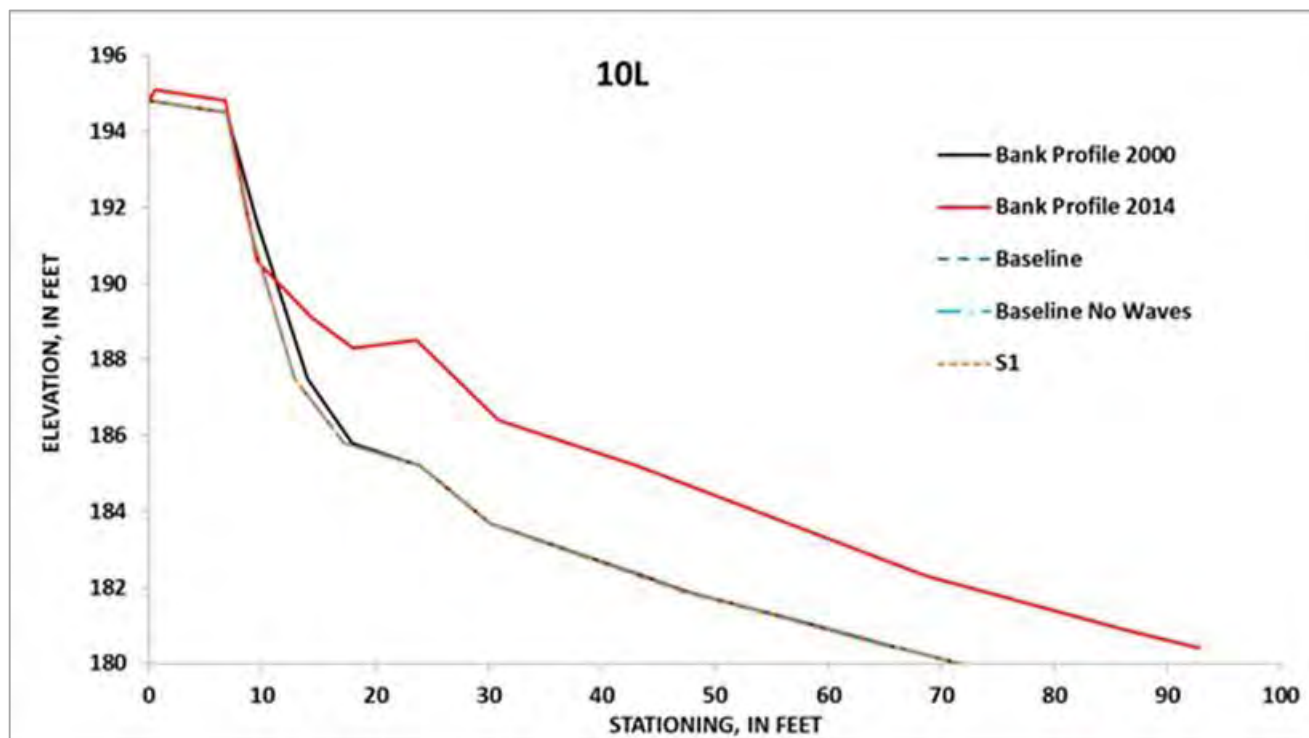
Figure 5.4.3.14-3: Simulated, future erosion for the Baseline Condition (with boat waves on and off) and Scenarios 1 at site 10L for the period 2000-2014. Zoomed in at area of erosion for illustrative purposes.
