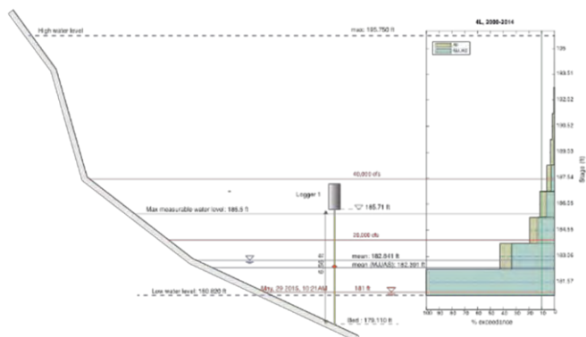
Figure 4.2.8.2-6 WLOG-1 installation elevation
