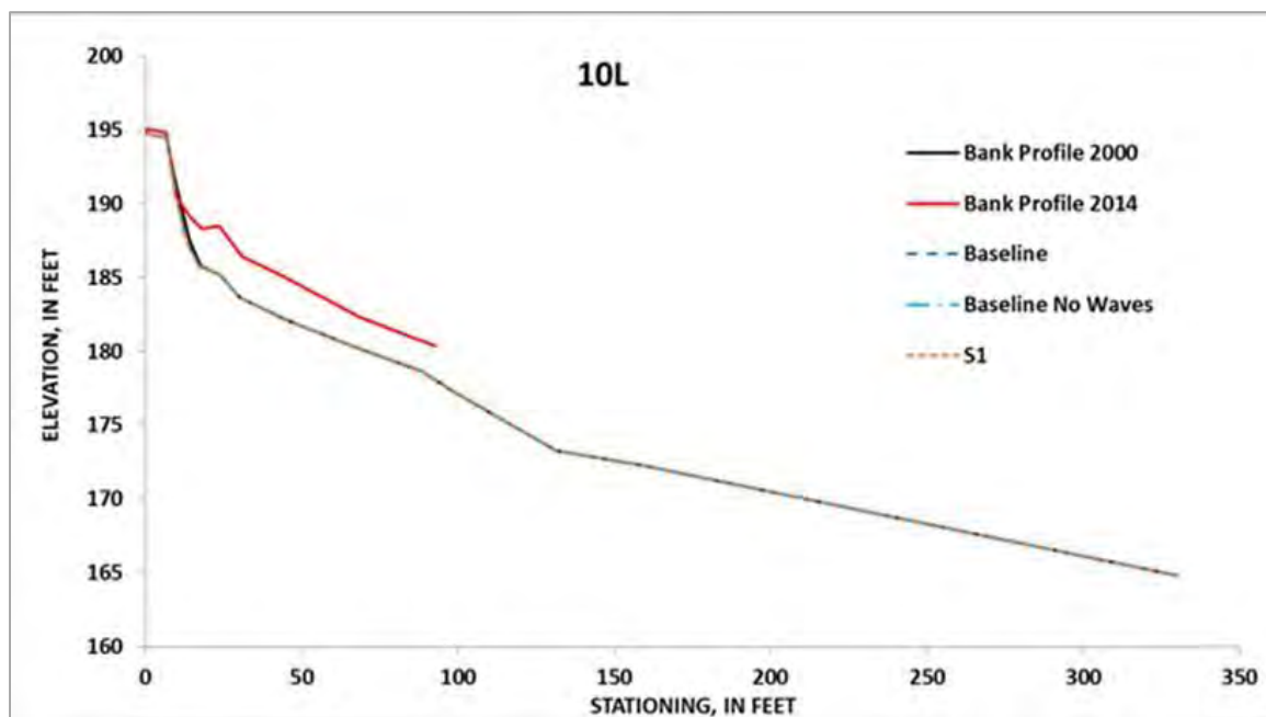
Figure 5.4.3.14-2: Simulated, future unit-erosion for the Baseline Condition (with boat waves on and off) and Scenario 1 at site 10L for the period 2000-2014
