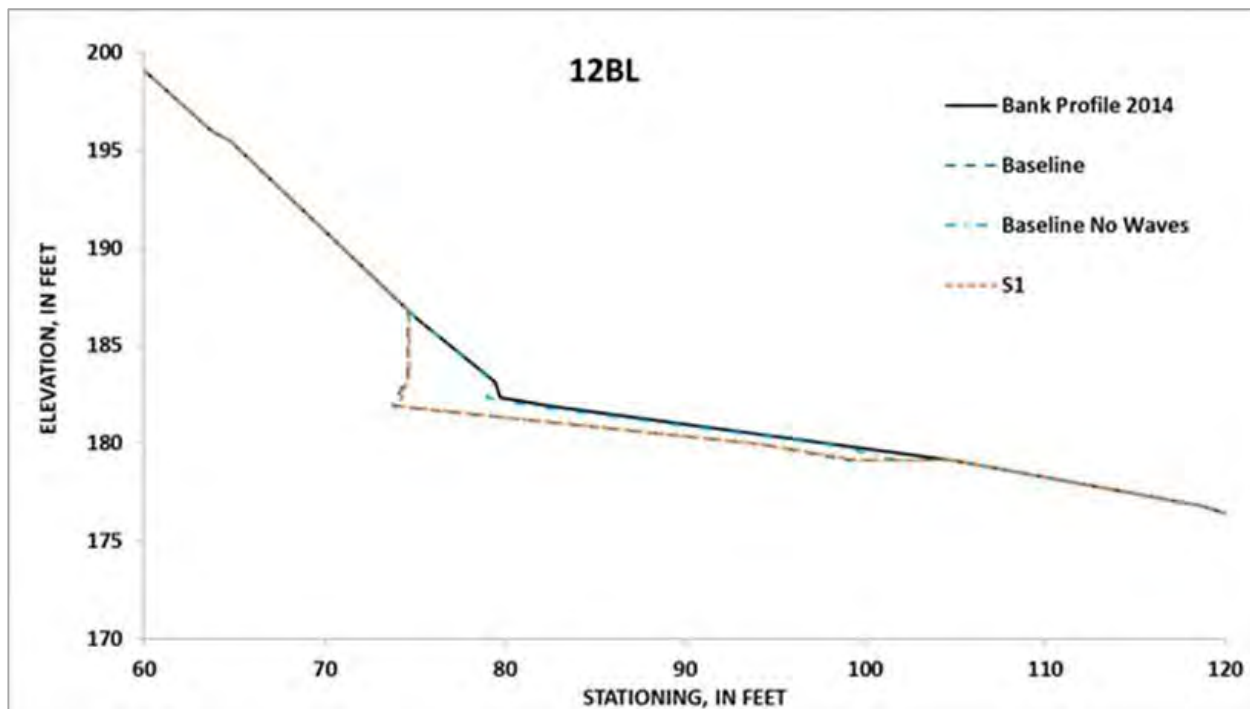
Figure 5.4.2.2-2: Example of the Important Effect of Boat Waves in the Lower TFI (Reach 1) showing the Greater amount of Hydraulic Erosion (Undercutting) between the Baseline Condition with Waves as Compared to the Baseline Condition Without Waves at Site 12BL
