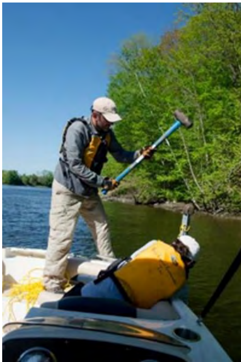
Figure 4.2.8.2-9: Installation of the T-posts
