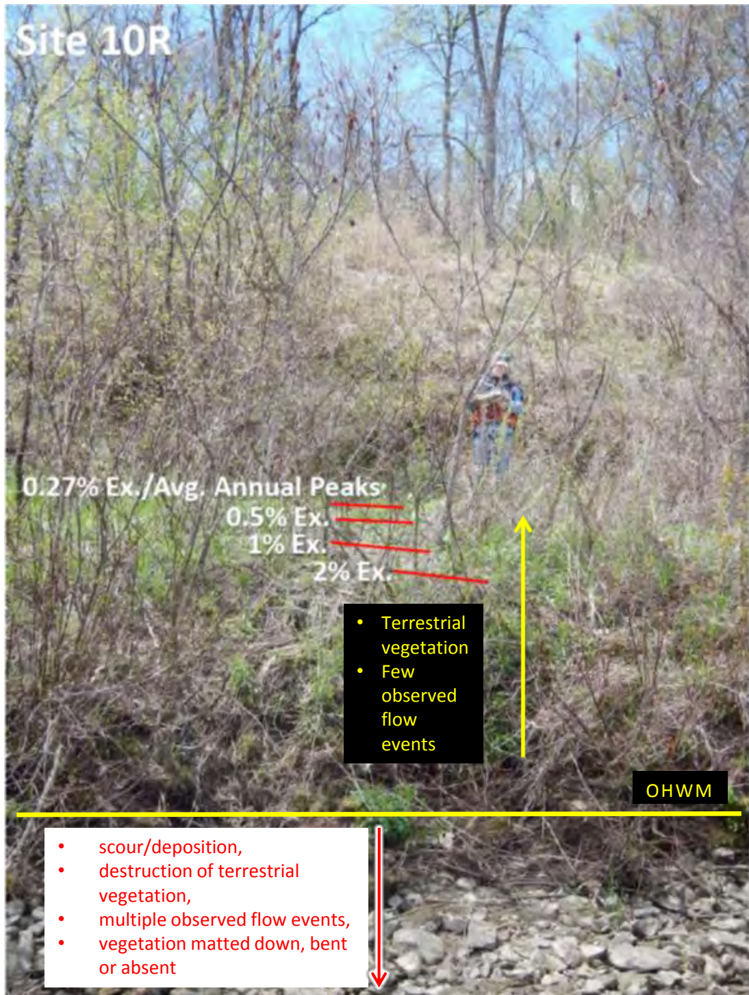
Figure 4.2.4.1-6 Physical characteristics of OHWM at Site 10R
