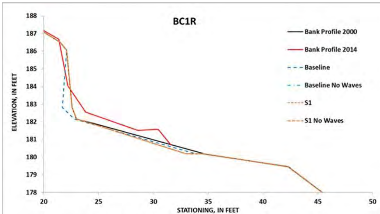
Figure 5.4.3.30-3: Simulated, future erosion for the Baseline Condition (with boat waves on and off) and Scenario 1 at site BC-1R for the period 2000-2014. Zoomed in at area of erosion for illustrative purposes
