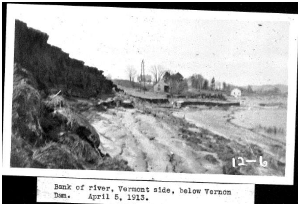
Figure 5.5.5.6 Eroded Bank in Turners Falls Impoundment Downstream of Vernon Dam – April 5, 1913 (TransCanada)
