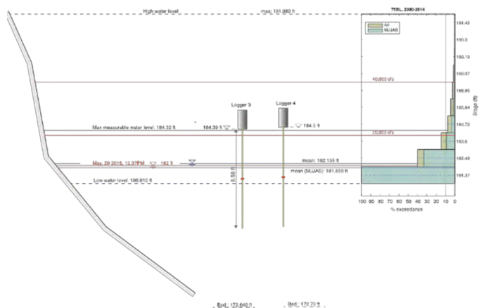
Figure 4.2.8.2-8 WLOG-3 and 4 installation elevation
